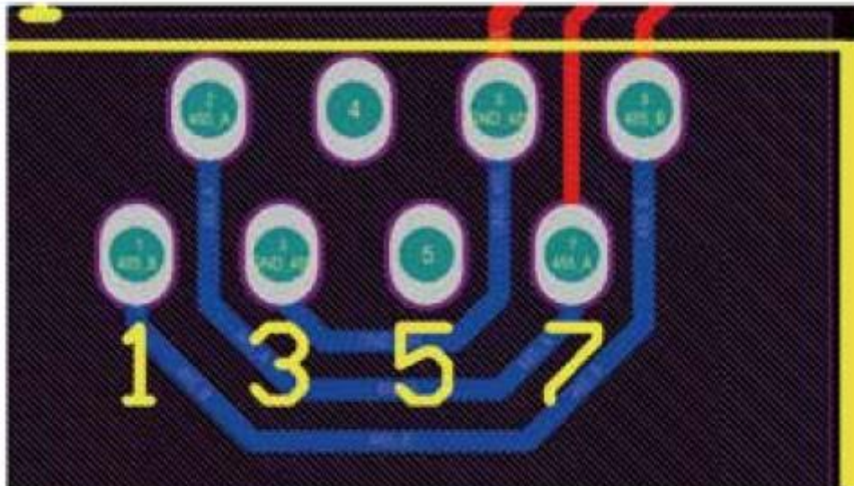
RS485 Port
